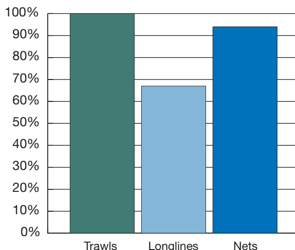
Figure 3.5 Percentage of chondrichthyan species ( n=71 ) within the Mediterranean, for which bycatch in trawls, longlines and nets, pose a major threat.
